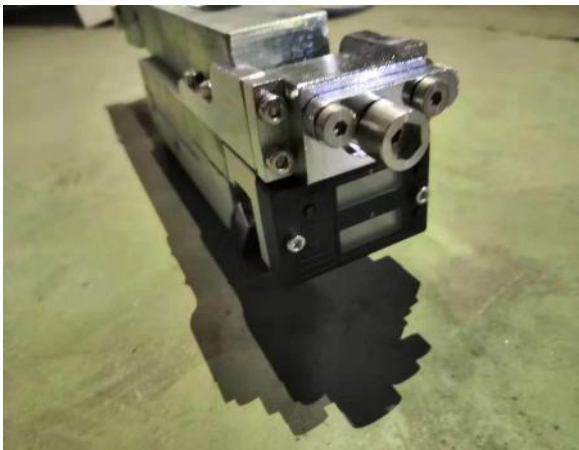
Grooving knife holder with digital indicator
