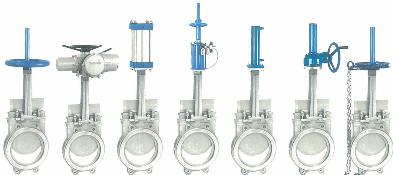
手动 Handle Wheel Knife gate valve
