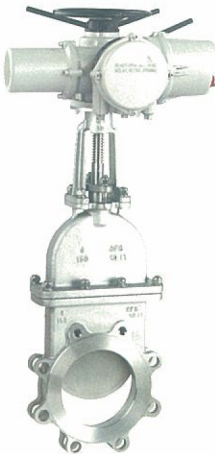
电动 Electric actuated Knife Gate Valve
