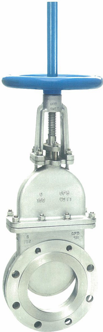
手动 Handle Wheel Knife gate valve
