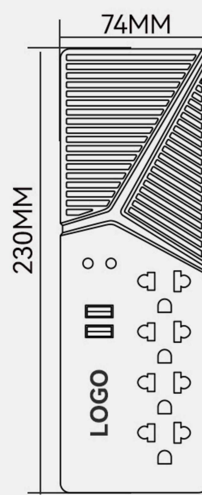
FRONT VIEW
